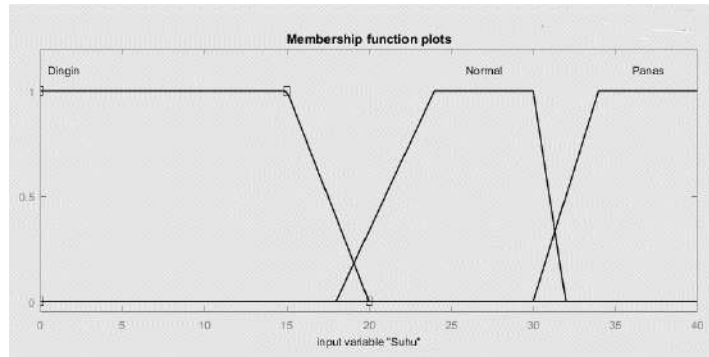
Figure 10. Membership Temperature
