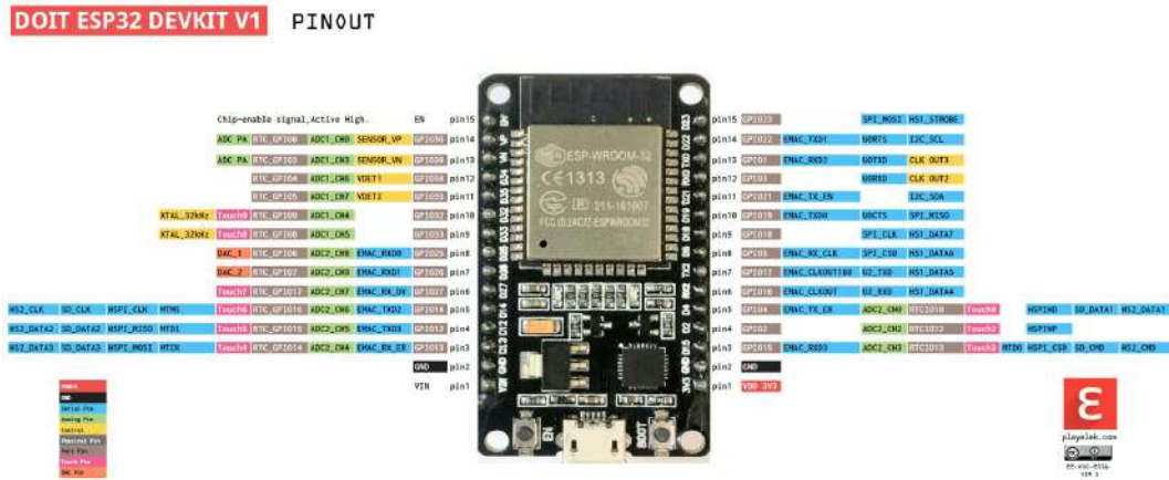
Figure 1. ESP32
