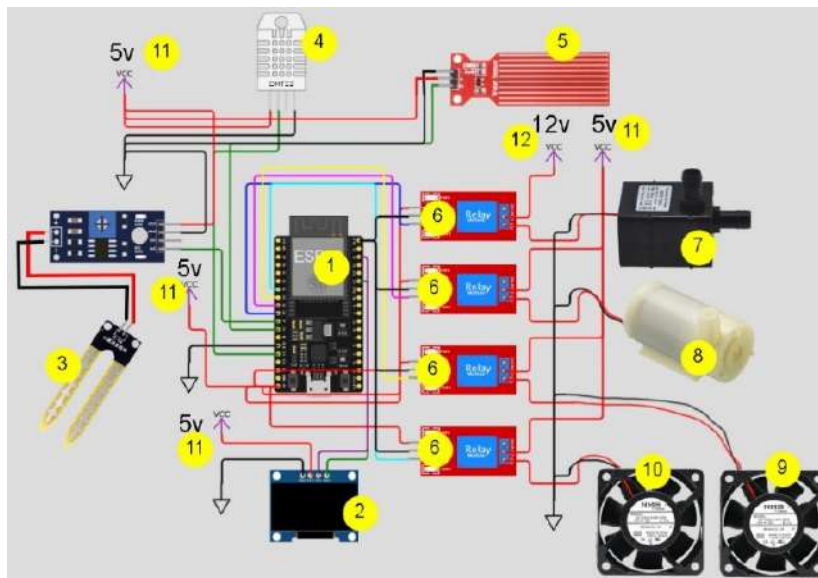
Figure 8. System Design
