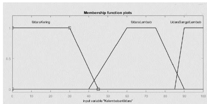
Figure 11. Membership Humidity
