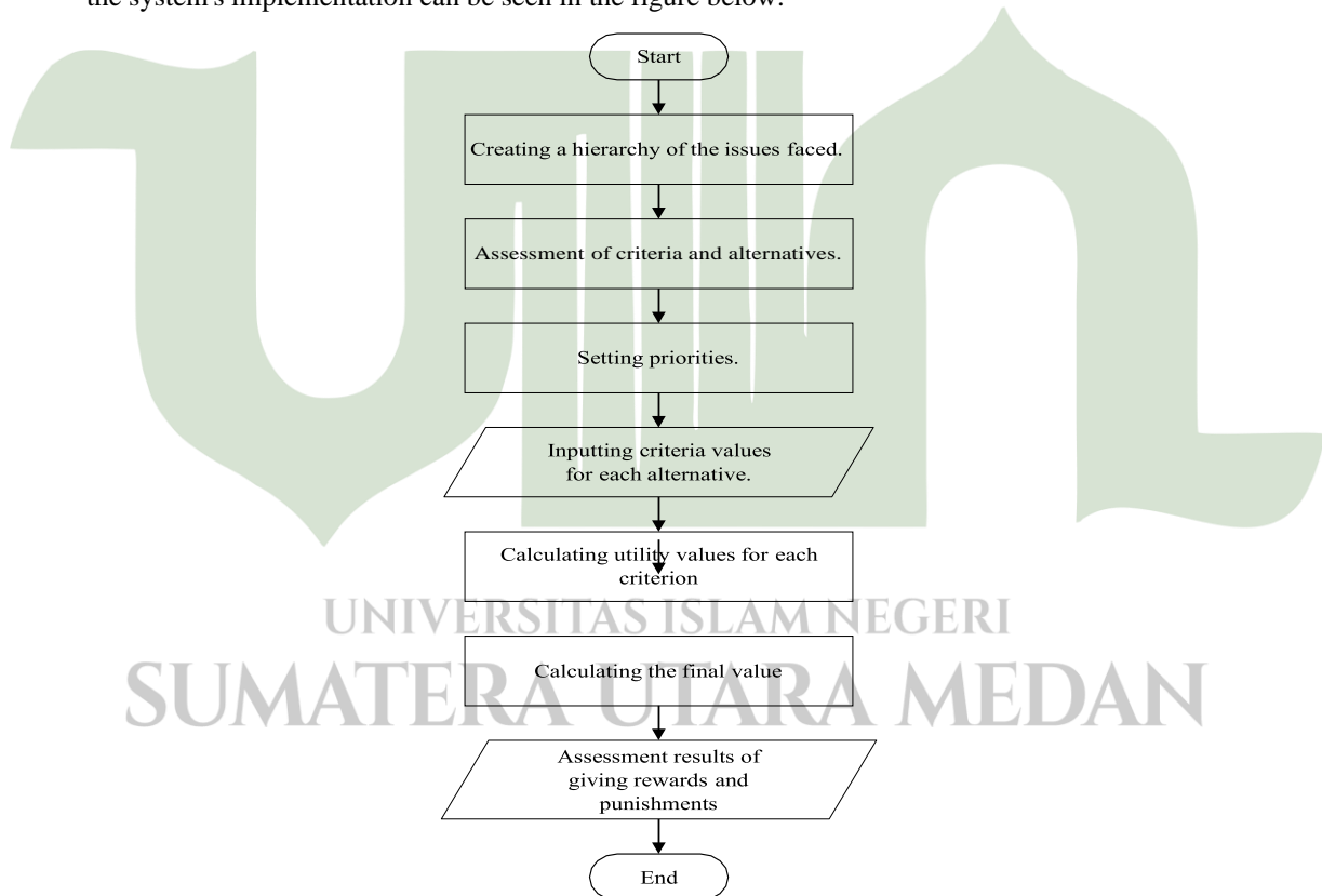
Figure 2. Flowchart of AHP and SMART Method
