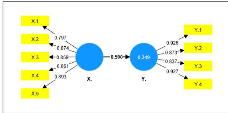
Figure 1. PLS Algorithm Source: SmartPLS 4.0 (2023)
