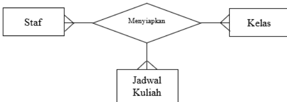
Gambar 4.8. Ternary
