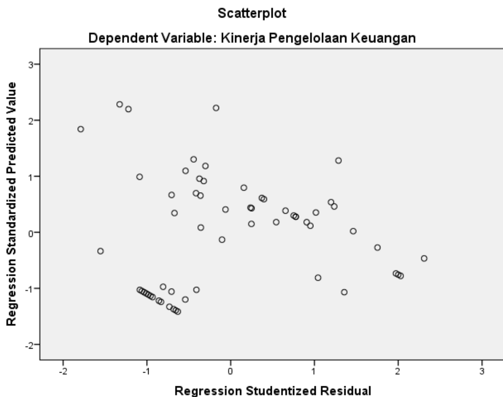
Gambar 4.4 Scatterplot
